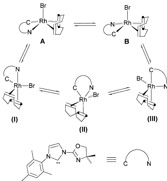
Scheme 3. A sequence of Berry pseudo-rotations leading to the exchange of the positions of the \text{C}=\text{C} double bonds in the chelating diolefin ligands relative to the \text{C,N} bidentate ligand. This process, together with the dissociation and re-association of \text{Br}^- , explains the exchange pattern observed in the variable temperature ^1\text{H} NMR spectra of 3 and 4
