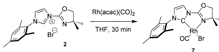
Scheme 6. Synthesis of the neutral four-coordinate complexes [RhBr(ligand)(CO)] ( 7 )
