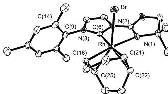
Figure 1. Molecular structure of 3 ; selected bond lengths (Å) and angles (°): Rh–Br 2.7545(3), Rh–N(1) 2.255(2), Rh–C(6) 2.022(2), Rh–C(18) 2.090(3), Rh–C(25) 2.096(3), Rh–C(21) 2.223(2), Rh–C(22) 2.251(2), C(21)–C(22) 1.371(4), C(18)–C(25) 1.428(4); C(6)–Rh–N(1) 77.47(9), C(6)–Rh–Br 86.98(7), N(1)–Rh–Br 81.89(6)(4)
