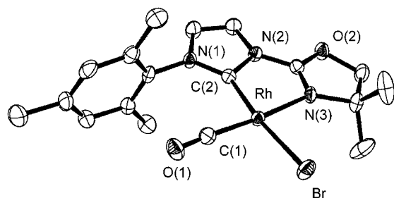
Figure 7. Molecular structure of 7 ; selected bond lengths (Å) and angles (deg): Rh–Br 2.5072(5), Rh–C(1) 1.807(4), Rh–C(2) 1.950(4), Rh–N(3) 2.143(3), C(1)–O(1) 1.152(4); Br–Rh–C(1) 90.1(1), Br–Rh–C(2) 173.0(1), C(2)–Rh–N(3) 78.4(1).
