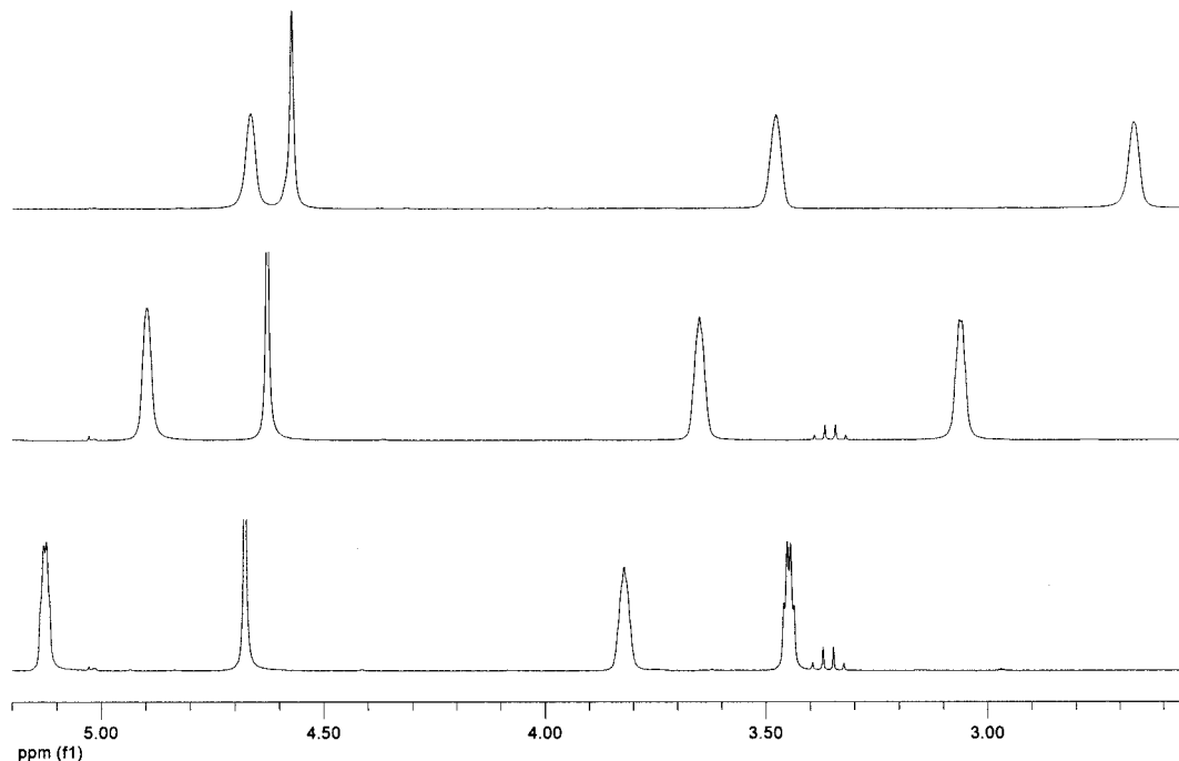
Figure 6. ^1\text{H} NMR spectra of complex 4 (top), a 1:1 mixture of 4 and 6 (middle) and 6 (bottom) recorded in \text{CD}_2\text{Cl}_2 at 203 K
