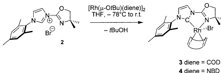
Scheme 2. Synthesis of the five-coordinate complexes [\text{RhBr}(\text{ligand})(\text{diene})] 3 and 4
