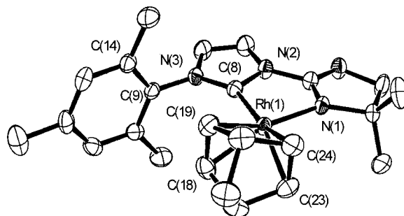
Figure 5. Molecular structure of 6 ; selected bond lengths (Å) and angles (°): Rh(1)–C(8) 2.039(6), Rh(1)–N(1) 2.120(5), Rh(1)–C(18) 2.098(7), Rh(1)–C(19) 2.106(7), Rh(1)–C(23) 2.196(7), Rh(1)–C(24) 2.189(7), C(18)–C(19) 1.38(1), C(23)–C(24) 1.35(1); C(8)–Rh–N(1) 78.2(2), C(19)–Rh–C(24) 67.1(3)
