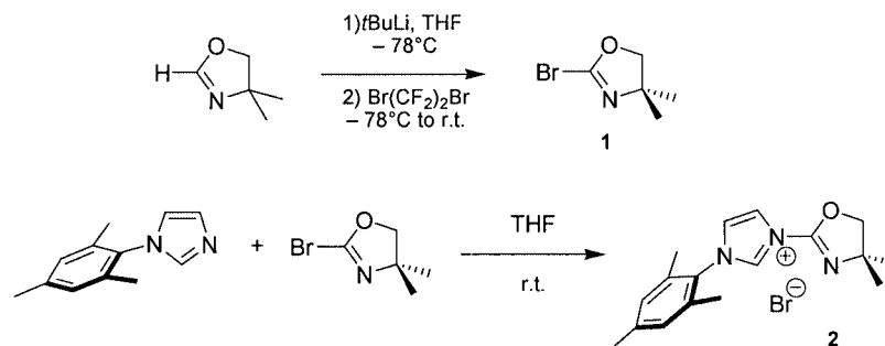
Scheme 1. Synthesis of the 2-bromooxazoline 1 and the oxazolinyl imidazolium salt 2 as ligand precursor
