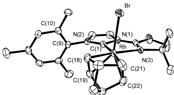
Figure 2. Molecular structure of 4 ; selected bond lengths (Å) and angles (°): Rh–Br 2.7615(3), Rh–N(3) 2.178(2), Rh–C(1) 2.016(2), Rh–C(18) 2.070(2), Rh–C(19) 2.105(3), Rh–C(21) 2.192(2), Rh–C(22) 2.177(2), C(21)–C(22) 1.357(5), C(18)–C(19) 1.401(4); C(1)–Rh–Br 95.13(7), C(1)–Rh–N(3) 77.49(8), N(3)–Rh–Br 89.12(5)
