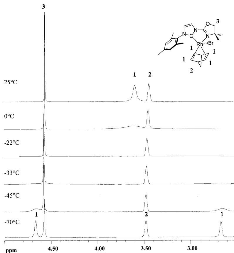
Figure 3. Variable temperature ^1\text{H} NMR spectra of 4 in the region \delta = 2.5\text{--}5.0 ppm (recorded in \text{CD}_2\text{Cl}_2 )
