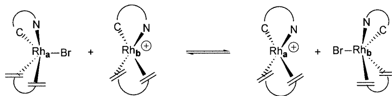
Scheme 5. Rapid intermolecular Br − exchange between complexes 4 and 6
