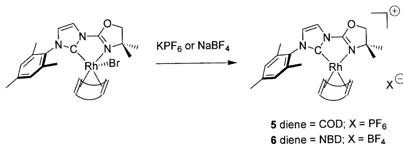
Scheme 4. Synthesis of the cationic four-coordinate complexes [\text{Rh}(\text{ligand})(\text{diene})]^+ 5 and 6
