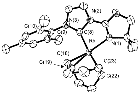
Figure 4. Molecular structure of 5 ; selected bond lengths (Å) and angles (°): Rh–N(1) 2.136(3), Rh–C(8) 2.037(7), Rh–C(18) 2.122(4), Rh–C(19) 2.116(4), Rh–C(22) 2.226(5), Rh–C(23) 2.206(5), C(18)–C(19) 1.371(7), C(22)–C(23) 1.357(8); C(8)–Rh–N(1) 78.7(2), C(18)–Rh–C(23) 81.5(2)
